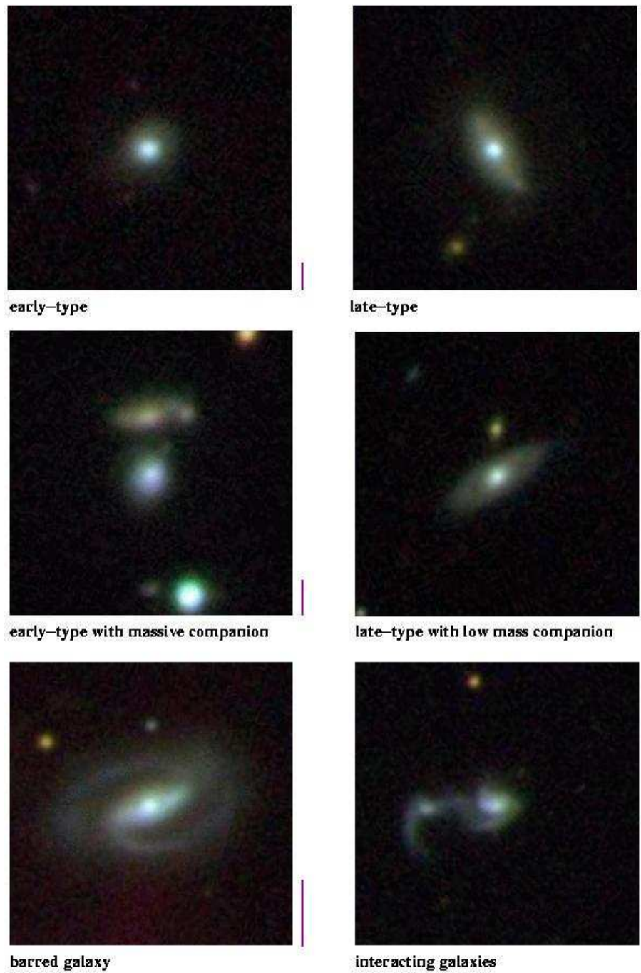
Figure 24: A montage of 48'' \times 48'' images of AGN with [OIII] luminosities greater than 10^{7.8} L_{\odot} . The purple bar next to each image is 10 kpc long at the redshift of the AGN.
